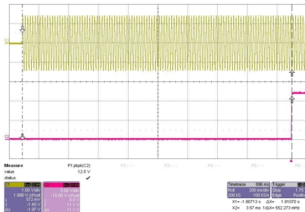
FS10-12 1.81S
