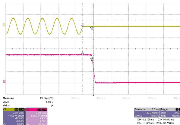
FS10-5 10.4mS
