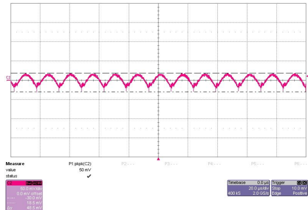
FS10-5 48.5mVpp
