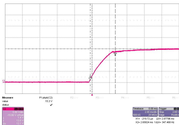
FS10-15 2.88mS
