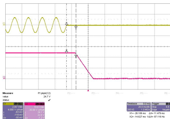
FS10-24 11.5mS
