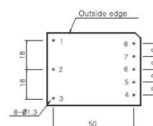
※ Mounting hole top view
