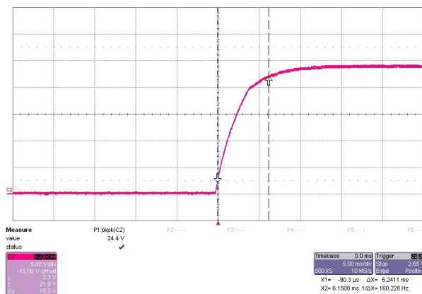
FS10-24 6.24mS
