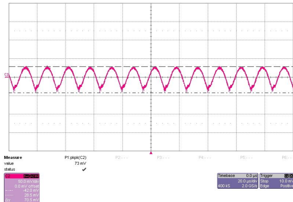
FS10-3R3 70.5mVpp
