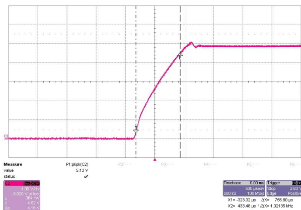
FS10-5 0.76mS
